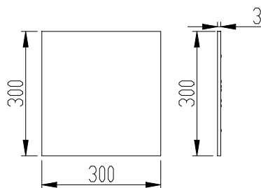
( figure 4 ) Aluminum Radiator Size
